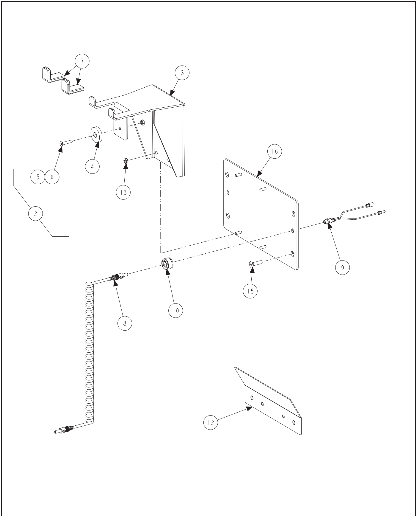
STORAGE KIT, 20-2380-1 REFER TO NEXT SHEET FOR PARTS DESCRIPTION LISTING
