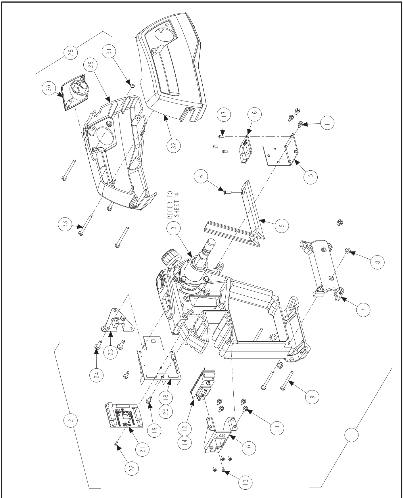
DSP700 SENSOR ASSEMBLY REFER TO NEXT SHEET FOR PARTS DESCRIPTION LISTING
